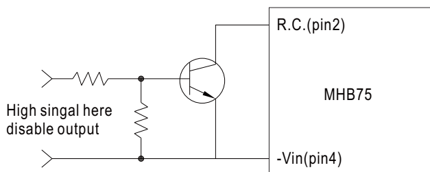
Example control circuit(positive logic)
