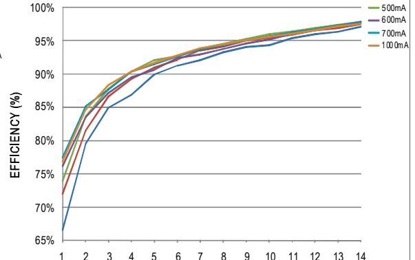
Fig-4 48VDC input, 1~14 LEDs (Vf=3V)
