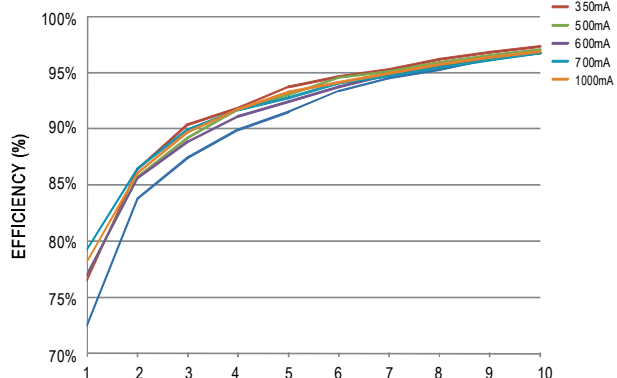
Fig-3 36VDC input, 1~10 LEDs (Vf=3V)
