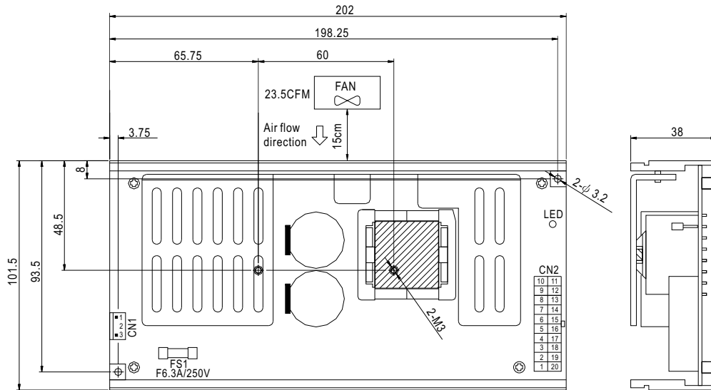
AC Input Connector (CN1) : JST B3P-VH or equivalent
